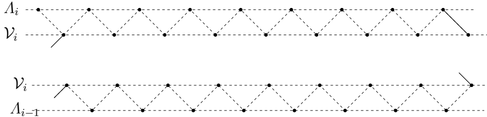
FIGURE 7.5. The two kinds of slices
