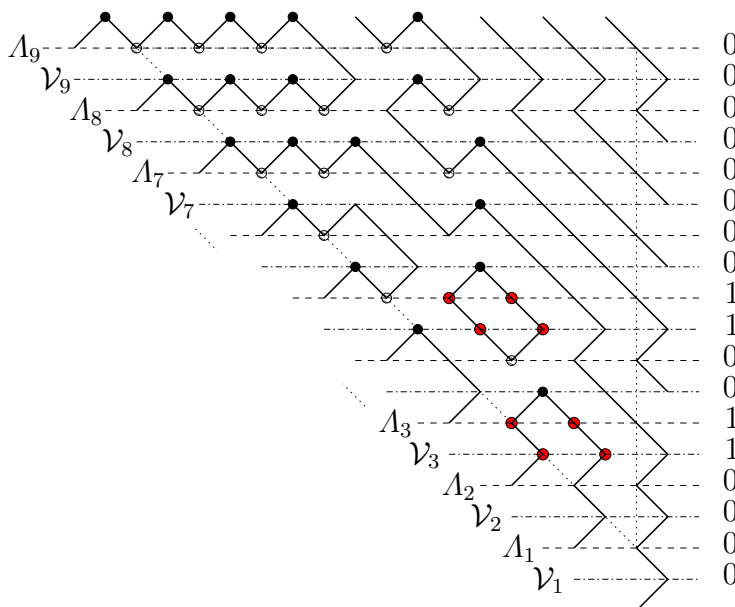
FIGURE 7.3. The region \mathcal{R} after rotation
