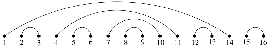
FIGURE 2.2. A planar matching
