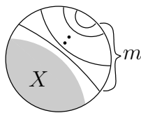
FIGURE 1.4. The matching composed out of a matching X and m nested arches
