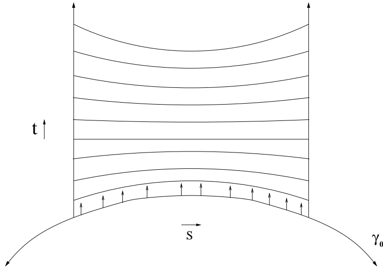
FIGURE 1. Geodesic variation.
