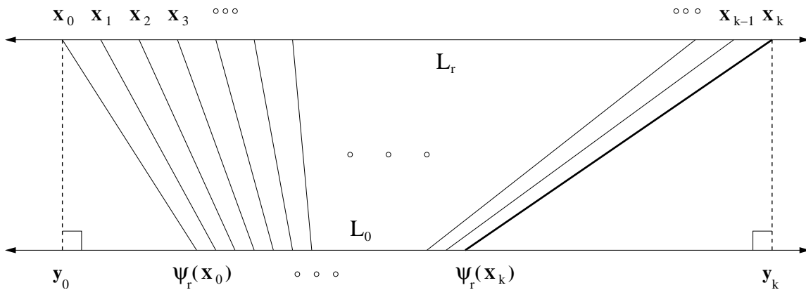
FIGURE 5. Illustration of the proof of our Assertion .
