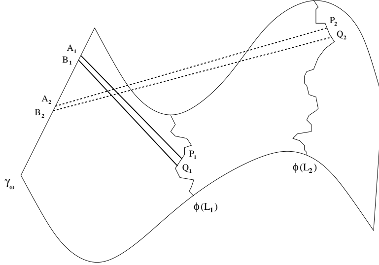
FIGURE 6. Choosing the points \{A_j, B_j, Q_j, P_j\} .
