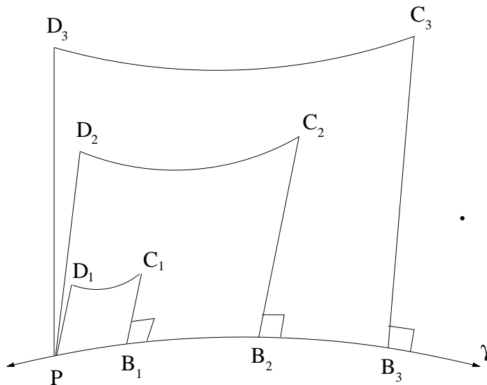
FIGURE 2. Pointed flattening sequence along a geodesic.
