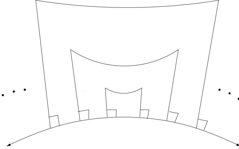
FIGURE 3. Flattening sequence along a geodesic.
