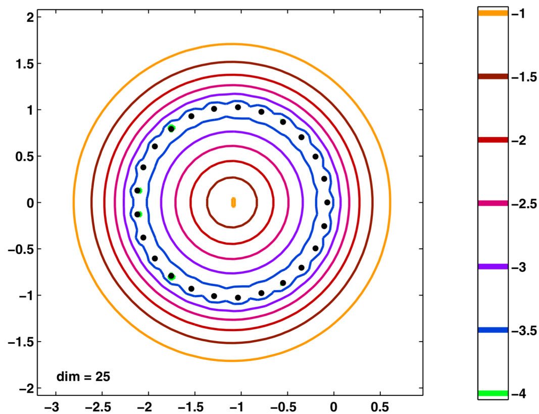
Fig. 4 \epsilon -pseudospectra for the transient example.
