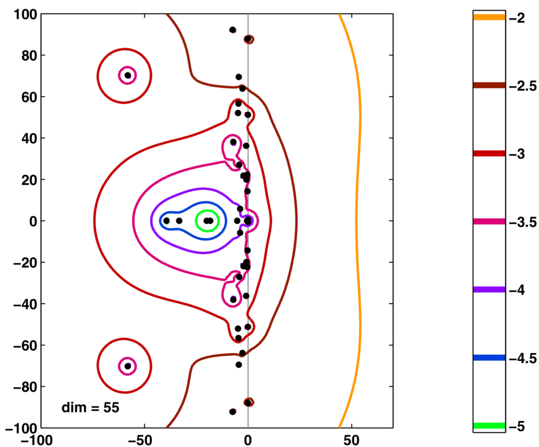
Fig. 6 \epsilon -pseudospectra for the stabilized Boeing 767.
