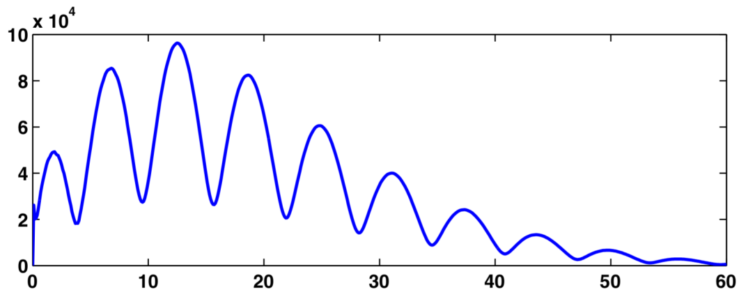
Fig. 5 \|e^{tA}\| , the hump for the stabilized Boeing 767.
