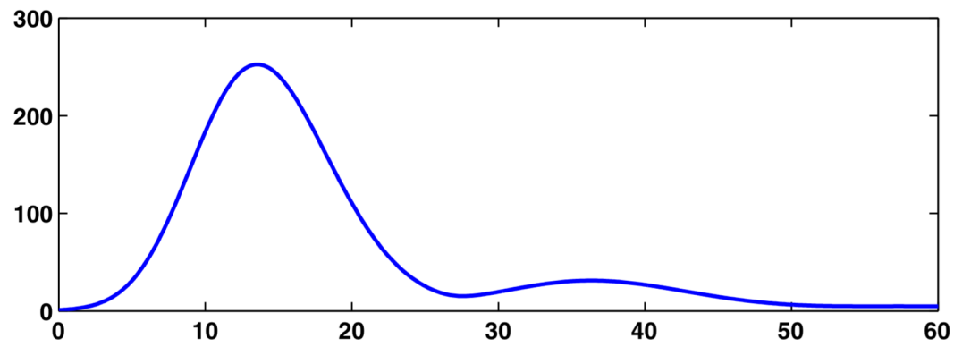
Fig. 3 \|e^{tA}\| , the hump for the transient example.
