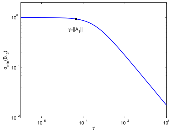
FIG. 4.1. Value of \sigma_{\min}(\widehat{B}_{12}) as \gamma varies (cf. Proposition 4.1).
