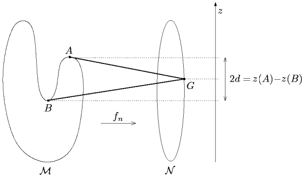
Figure 4 An example of a train of limit d -jumps given by the triple (B, G, A) .
