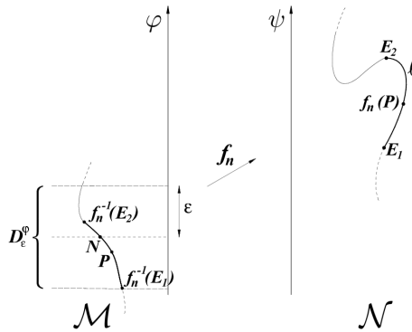
Figure 5 In this example a connected component \ell of the set f_n(D_\varepsilon^\varphi) - K_\psi , containing P , is represented on the right (thick line).
