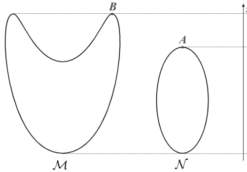
Figure 1 The natural pseudo-distance between the size pairs (\mathcal{M}, z) and (\mathcal{N}, z) is z(B) - z(A) .
