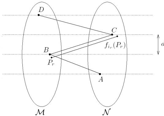
Figure 3 A train of limit d -jumps given by the quadruple (A, B, C, D) .
