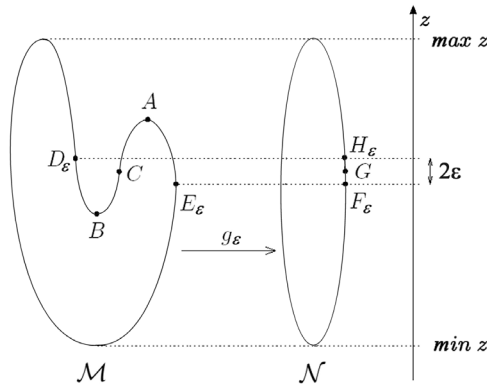
Figure 2 Construction of the homeomorphism g_\epsilon for which \Theta(g_\epsilon) \leq d + \epsilon .
